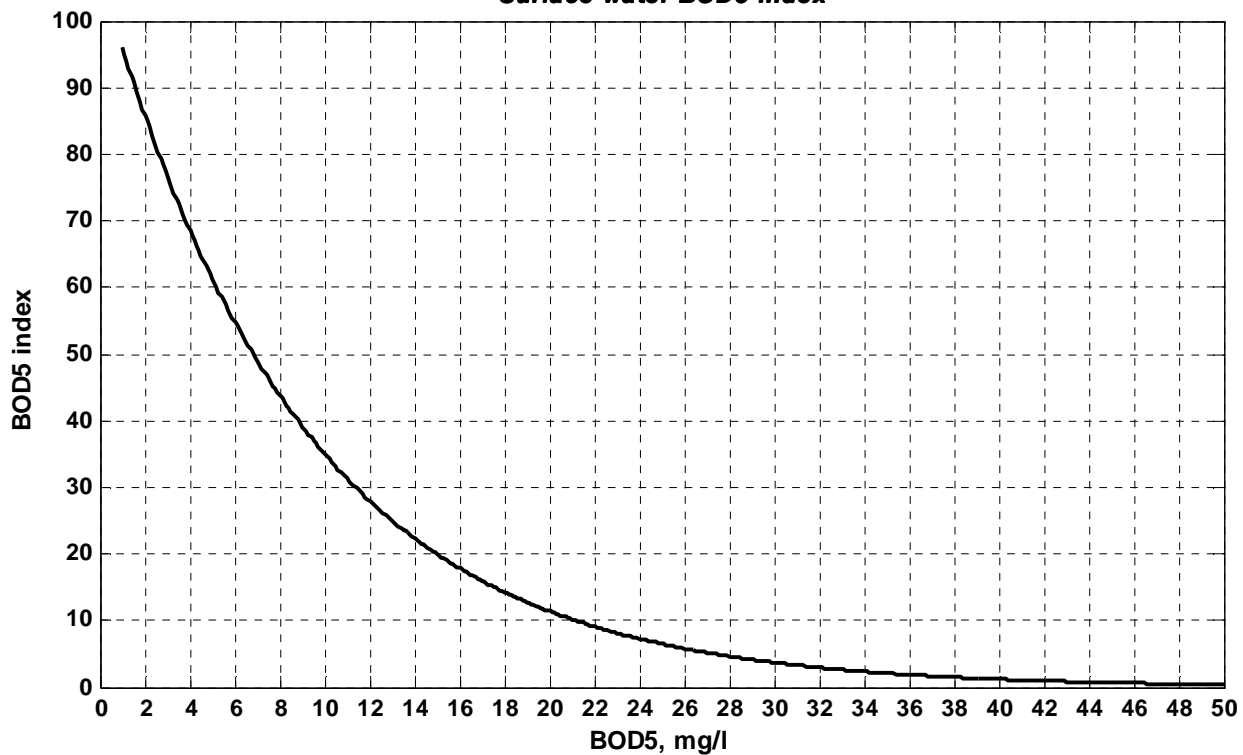
Surface water BOD5 index
