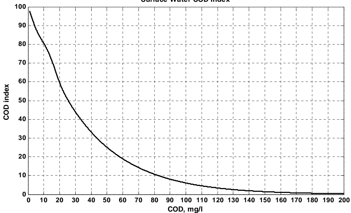
Surface Water COD Index
